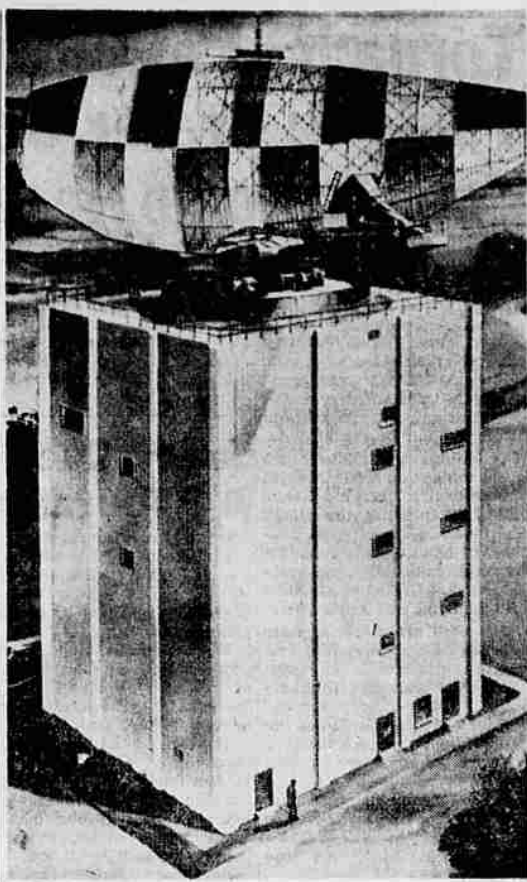
RADAR TOWER - This artist's conception depicts a radar tower which will be installed at Point Arena Radar Site, north of San Francisco, early this spring. It has been announced by the Air Force. The 84-foot, five story concrete building will house electronic equipment for new long range air defense radar and also double as an antenna base. The mammoth antenna system, including pedestal, fog horn and reflector, will be one of the world's largest rotating structures. (UPI Telephoto)
