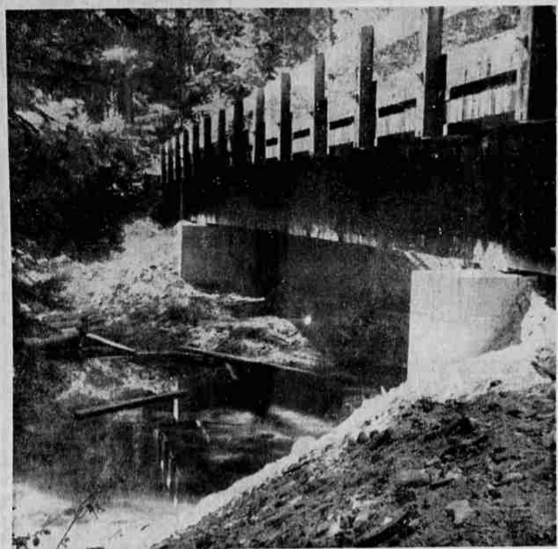
NEW BRIDGE - Recently completed was by two glue laminated beams. The super structure is all wood, with the exception of steel plate tread ways. Timber used was The forest access road bridge is supported all creosote treated. (BLM Photo)
