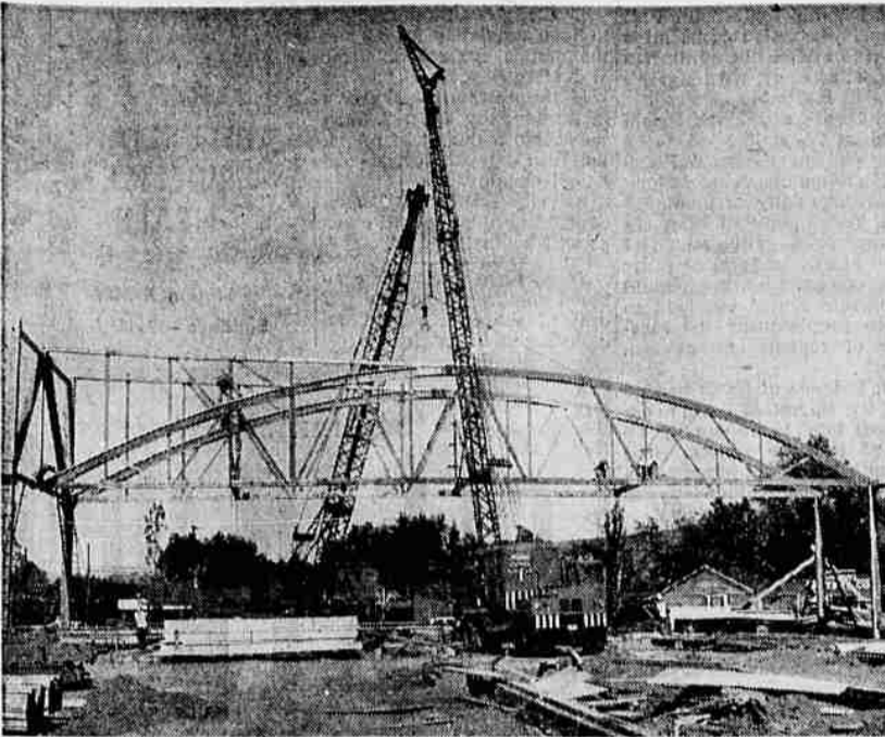
BEAMS INSTALLED—Cranes place beams in place on the new Medford Corporation plywood plant...
