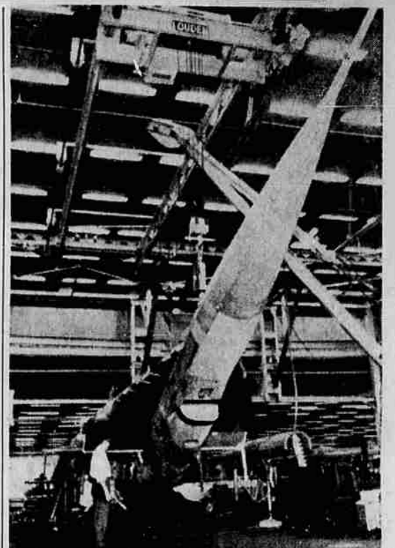
DRONE WEIGHED —Suspended from the ceiling, the SD4 Swallow, one of the Army's new battlefield surveillance drones, is carefully lowered onto scales for weighing at Republic Aviation plant at Farmingdale, N.Y. The weighing was to determine the Swallow's precise center of gravity, both vertically and horizontally. The information is necessary before electronic and avionic gear can be installed in the 30-foot all-weather drone that's designed to act as an "aerial spy". (UPI Telephoto)
