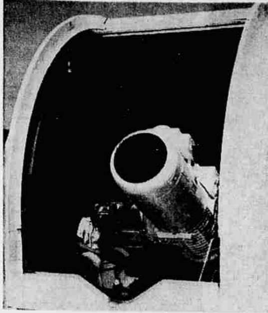
TELESCOPE CAMERA — The giant camera known as ROTI (Recording Optical Tracking Instrument) is operated by RCA under contract to the U.S. Air Force. The ROTI is basically a 24-inch telescope with a 500-inch focal length lens system coupled to a 70 millimeter camera with a film capacity of 1,000 feet. Two ROTI units are operated at Cape Canaveral and one down range. Air Force Ballistic Missile Division and Martin Company engineers use ROTI film sequence for missile performance evaluation. (UPI Telephoto)
