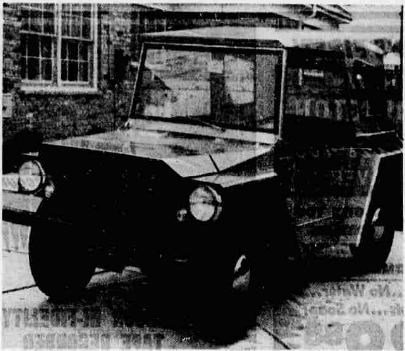
AUTOMOTIVE ENTRY — Latest entry in the automotive field is the "Scat", a lightweight utility vehicle announced by Saviano Vehicles of Warren, Mich. A two-door, four-passenger vehicle with an 80-hp wheelbase, the Scat has a 25-horsepower air-cooled front-mounted engine. Top speed is 50 miles per hour and fuel economy is between 25 and 30 miles per gallon. It is priced at $1,390, including delivery, handling and federal excise tax. — (UPI Telephoto)
