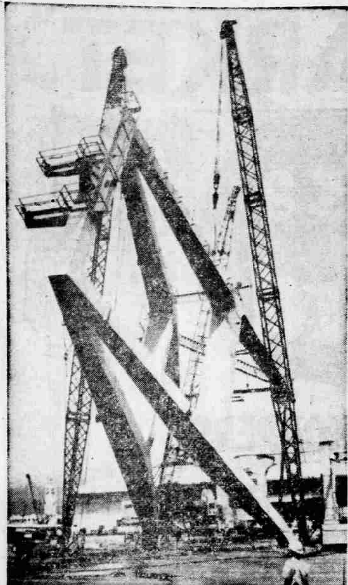
BIG JOB - One of the most intricate construction jobs in Hawaiian Island history took place at Honolulu this week at Pier 2, site of the first ship cargo container facility, when Biggs Crane and Rigging company of Oakland, Calif., made this 80-ton hoist. Aloft is a 130-foot A-frame section of Matson Navigation company's new $350,000 container crane. The day-long job was accomplished by means of towering section steel girders and 16 one-inch guy wires. The $4 million container facility is scheduled for mid-April completion. (UPI Telephoto)
