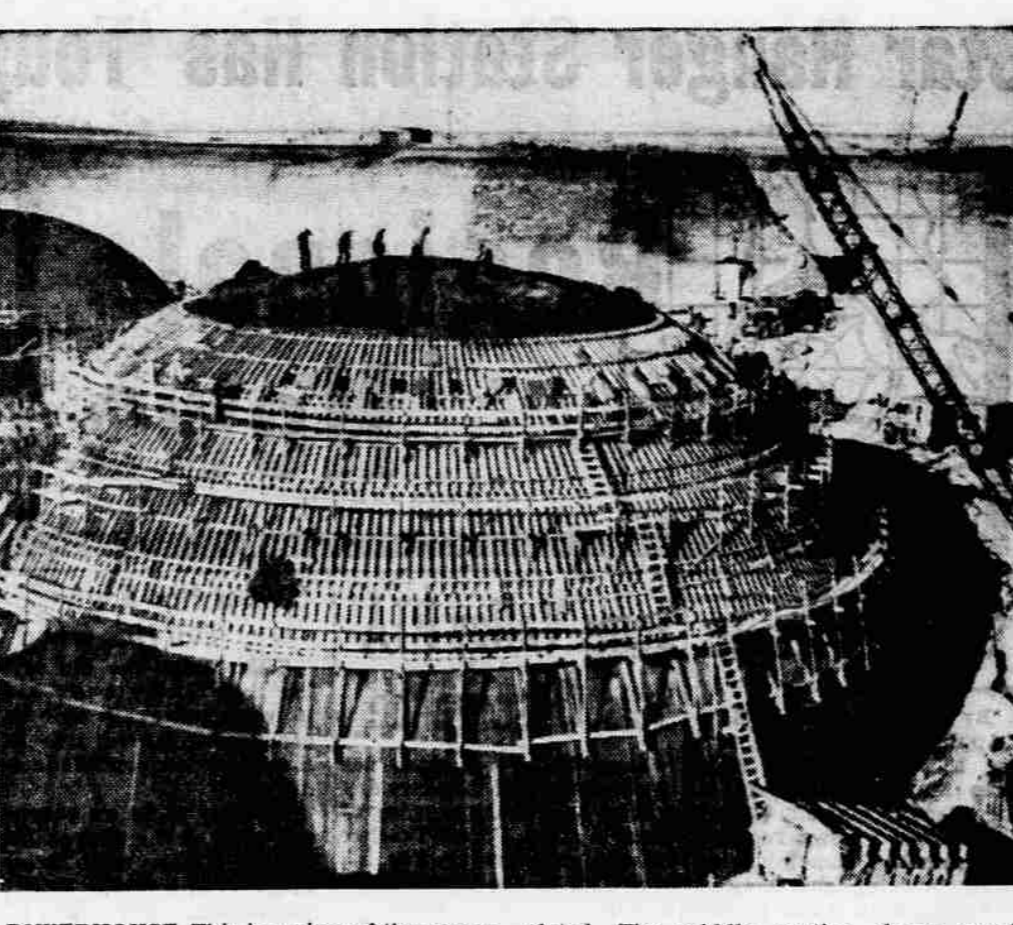
POWERHOUSE —This is a view of the powerhouse for the Air Force Titan ICBM base under construction by the Army Corps of engineers near Denver, Colo. At the base of the powerhouse, concrete work is completed. The middle portion shows wood framework for concrete which is being poured from the bucket at upper right. Men atop the dome are tying steel re-bars to strengthen concrete. (UPI Telephoto)
