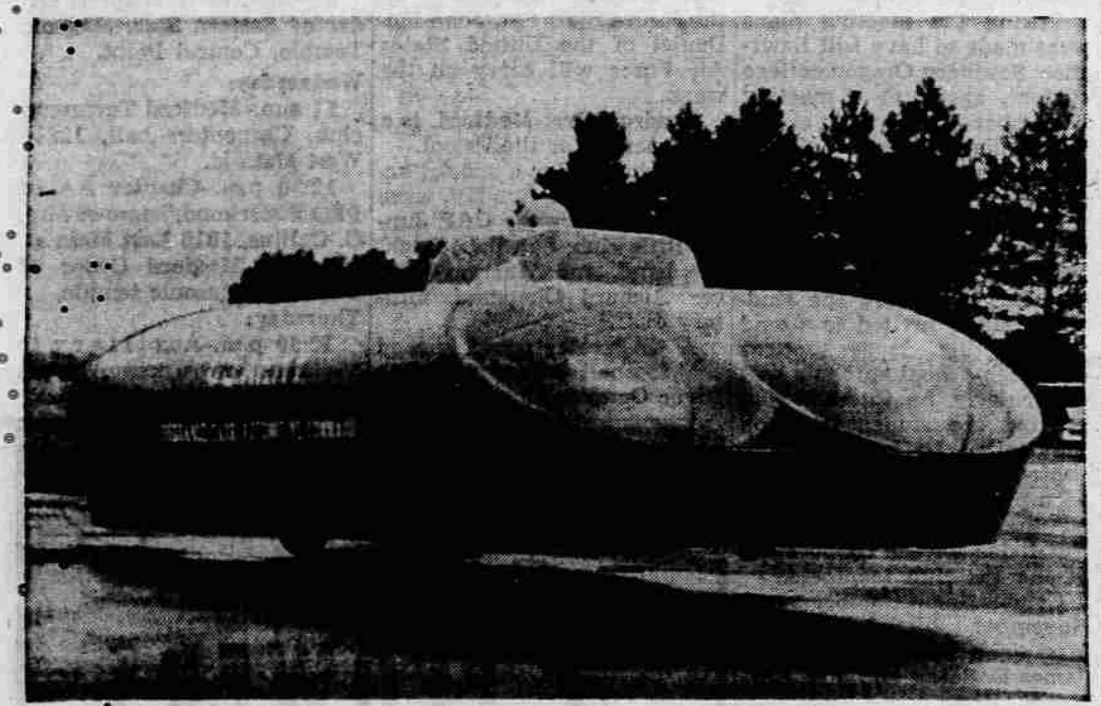
RIDING ON AIR—An Army flying saucer-type vehicle scoots across the ground during a demonstration at the "Symposium on Ground Effect Phenomena" at Princeton University. These flying machines operate a few inches above the ground on a cushion of air. The cushion is created by forcing air downward at great pressure, providing enough lift to raise the vehicle off the ground.
