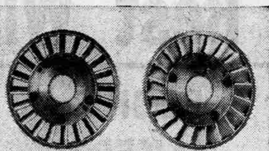
Economy Angle Performance Angle Nothing shifts but the pitch of the stator blades in a jet-smooth flow of oil. High angle for quick starts and passing. Low angle for economical cruising.
