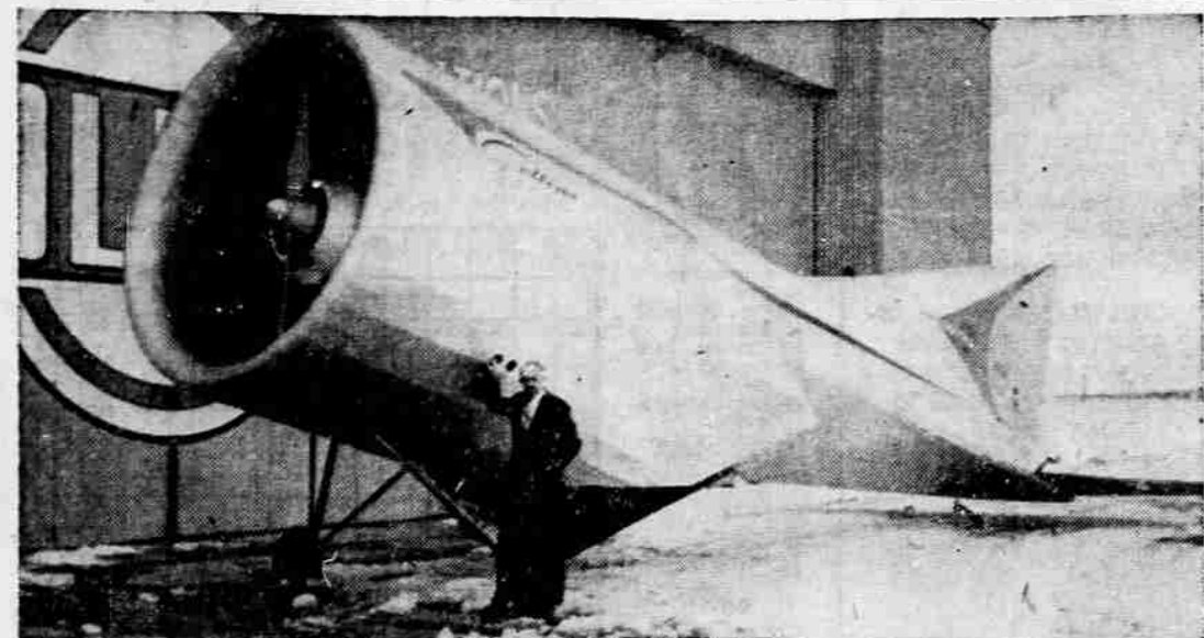
TAKING OFF WRAPS of radical new "Aerodyne" aerial vehicle, Dr. Alexander Lipisch, its designer, stands beside first full scale model at Cedar Rapids, Ia., plant where it was constructed. It is designed to take off vertically and achieve forward flight by channeling airflow from propellers internally through fuselage. Cockpit will be aft.
