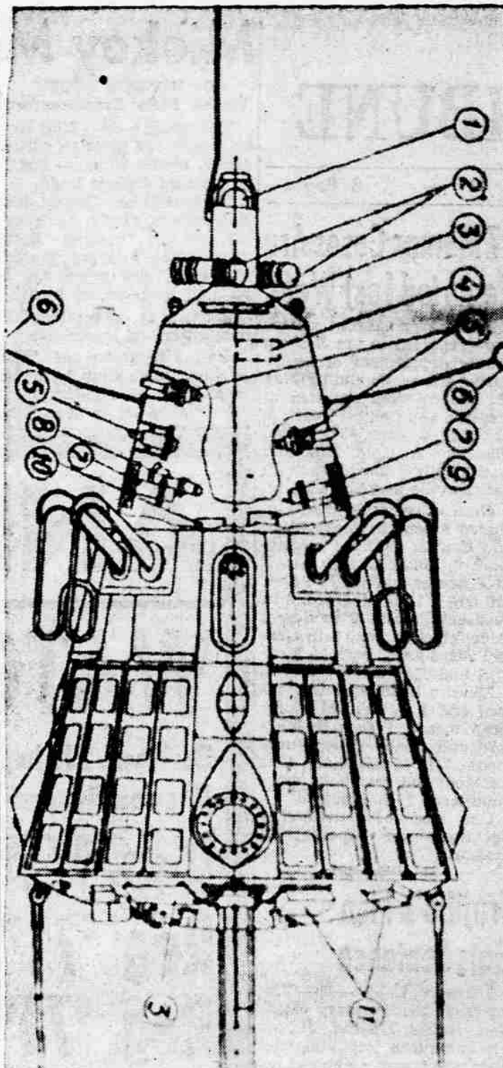
ANNOUNCING DETAILS of Sputnik III now orbiting earth, Moscow newspaper prints diagram of major features. 1, magnetometer; 2, fotomultipliers for measuring sun's radiations; 3, solar batteries; 4, instrument for recording photons and cosmic rays; 5, magnetic and ionization manometers; 6, ion traps; 7, electrostatic fluxmeters; 8, mass spectrometer cube; 9, instruments for recording heavy nuclei in cosmic rays; 10, instruments for measuring intensity of primary cosmic radiation; 11, instruments for recording micrometeors. (International Soundphoto)
