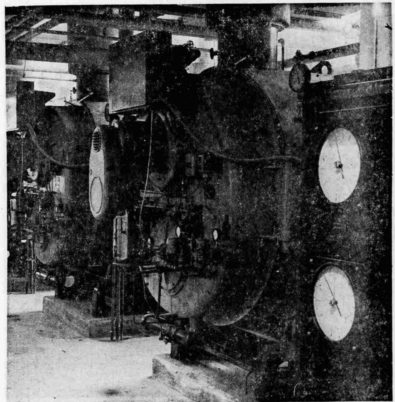
BOILERS TO FURNISH HEAT ARE AUTOMATIC
