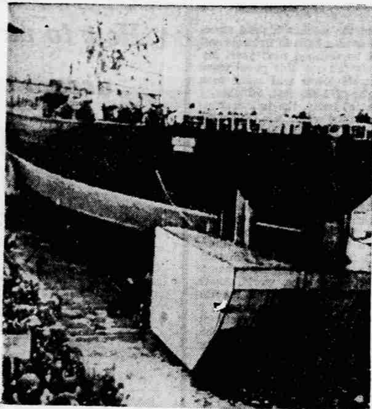
ATOMS AWEIGH —The world's first atomic-powered surface vessel, the ice-breaker Lenin, slides down the ways during launching by the Soviets at Leningrad. Statistics of the nuclear ship: 44,000 horsepower; 438-foot long; beam of 88 feet and a displacement of 16,000 tons.
