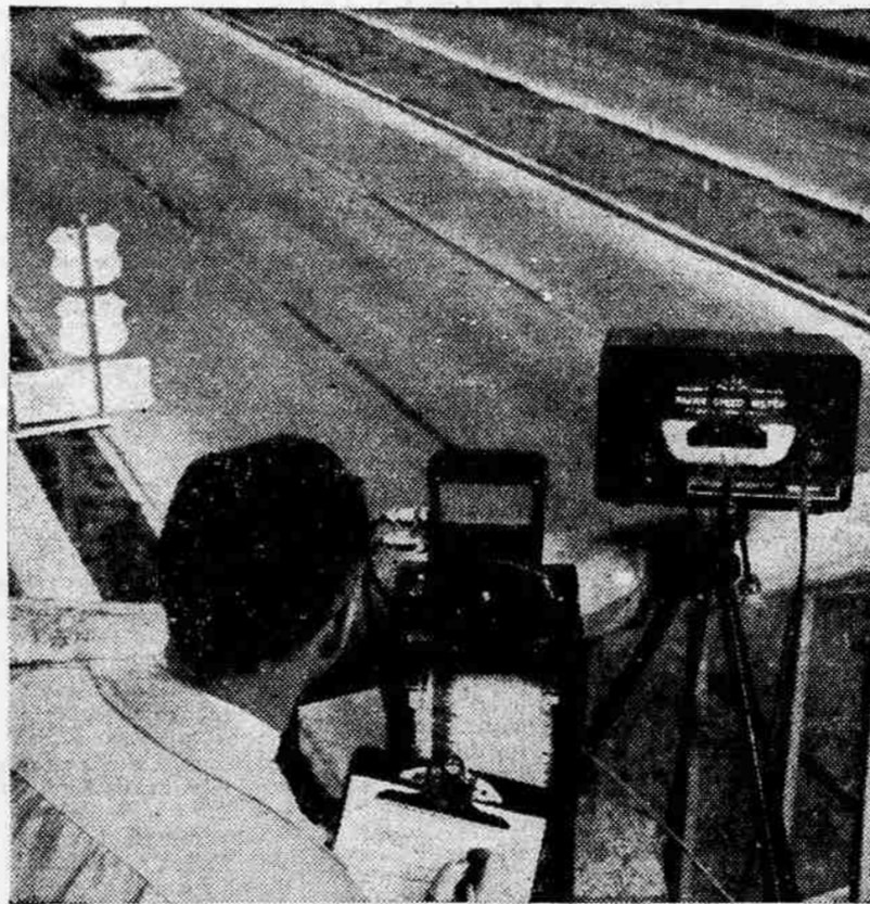
WITHOUT TCP
