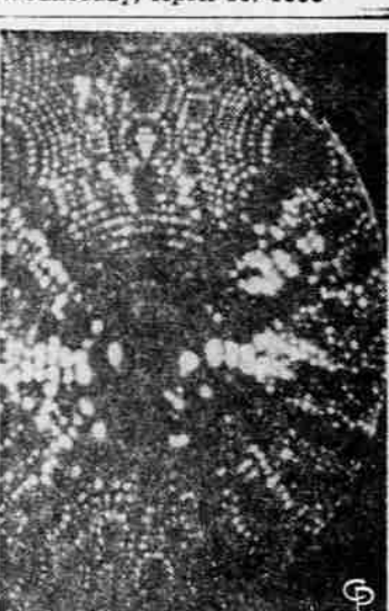
PHOTOGRAPHED for first time in history, atoms on surface of tungsten are seen by using filled ion emission microscope invented by Dr. Erwin W. Muller of Pennsylvania State University. Each dot represents single atom. Magnification is 2,750,000 times. (International)
