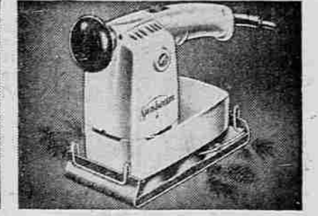
Sunbeam SANDER The Sander that stood up over 1000 hours in continuous use test. Saves time—gives professional results. Lightweight—only 4½ lbs.
