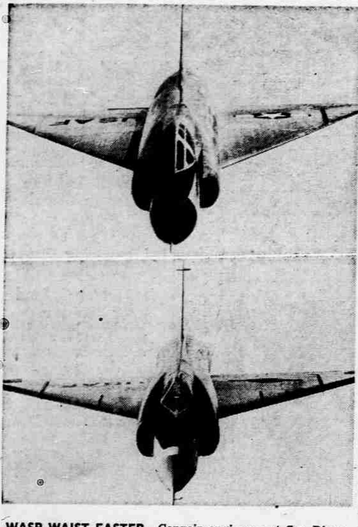
WASP WAIST FASTER —Convair engineers at San Diego have disclosed how they gave the F102A jet interceptor a wasp waist and increased its speed, allowing it to slip more smoothly through the sonic barrier. At top is the F-102 prototype with a straight fuselage, and at bottom is the F-102, with the pinched fuselage that reduces drag.
