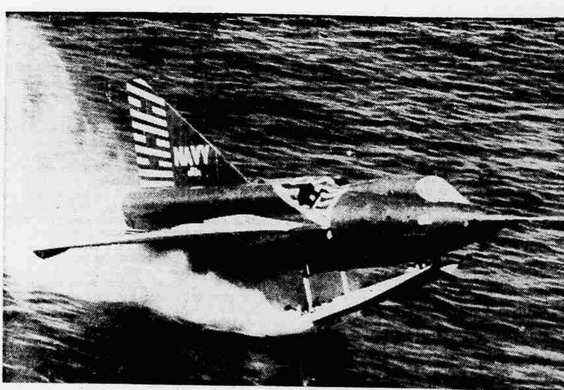
WELL-BALANCEU —The XF2Y-1 Sea Dart, Navy jet fighter, makes a high-speed taxi run at San Diego after being refitted with a single ski as part of the Convair-Navy hydrodynamic research program. The revolutionary plane, first jet seaplane ever built, has exceeded speed of sound.
