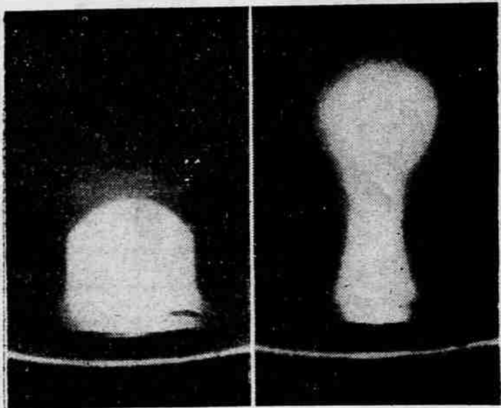
FLYING SAUCERS? ... COULD BE —These shining orange globes called "anode glows," produced in a partial vacuum with the aid of static electricity, are what Army physicist Noel W. Scott believes to be a miniature of conditions in the stratosphere responsible for "flying saucers." Scott produced the "things" in the Army laboratory at Ft. Belvoir, Va.
