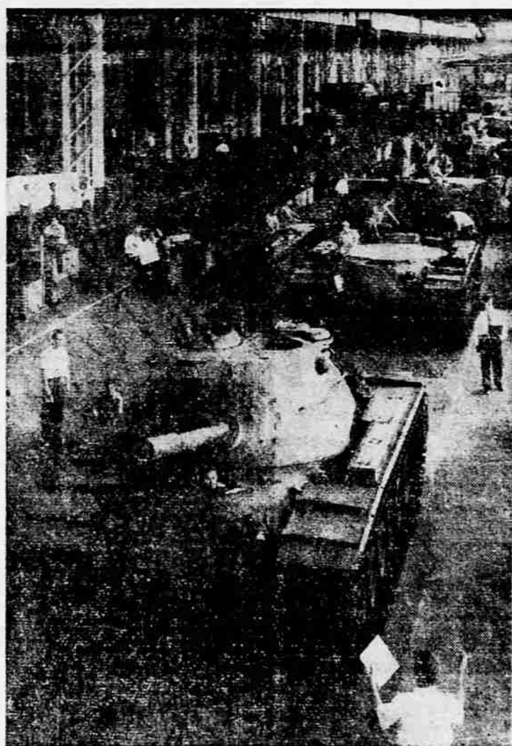
For the first time, the Army has permitted photographs of its new Patton 48 medium tanks rolling from the Chrysler Delaware Tank Plant assembly line. Military experts say this new spectacular tank will whip any other tank in the world. This million square foot tank plant pro- duced and delivered its first Patton 48 to Army Ordnance on April 11, 1952, less than a year from the date the first steel was raised.
