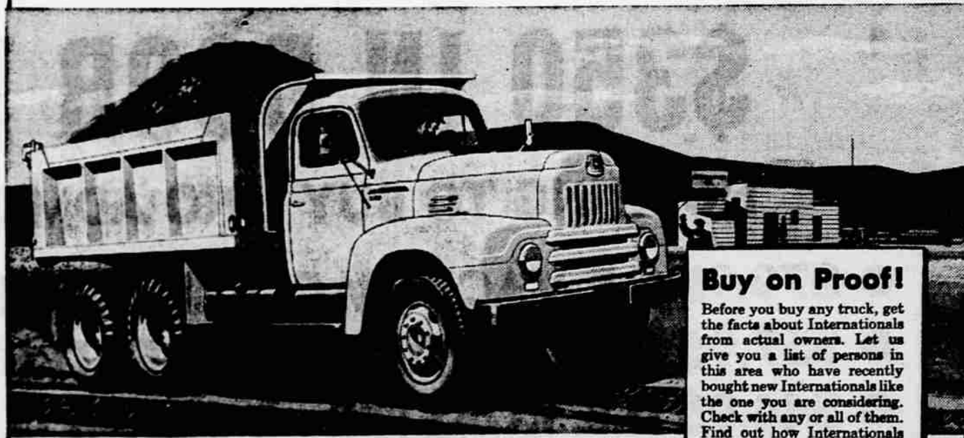
Model LP-310, 157-hp. wheelbase, 10 1/2 x 7-ft. dump body, 37,000 lbs. GVW.
