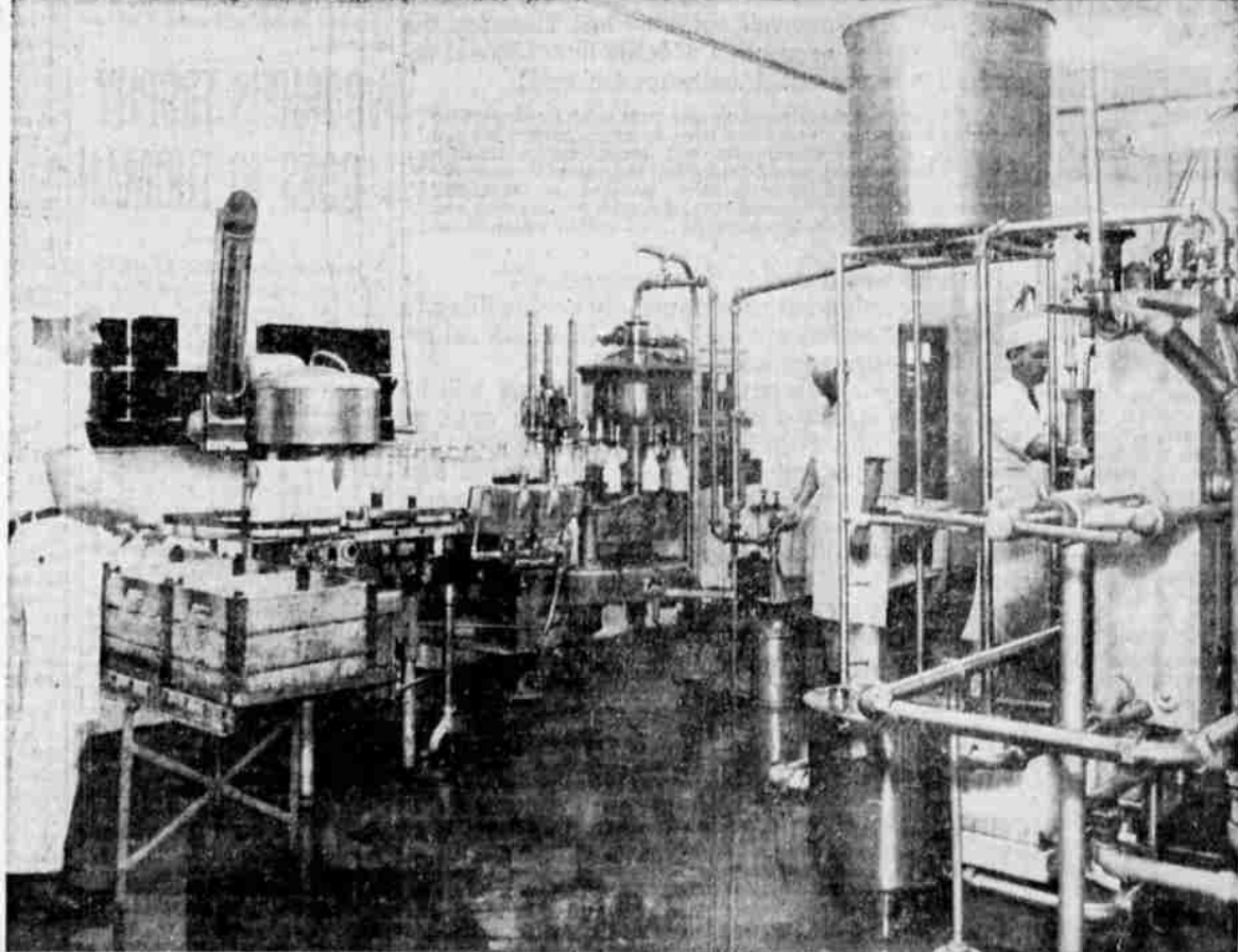
Top: Chery-Burrell Soaker-type Washer, which provides 12 separate washes for bottles. Center: Super-Plate Shorttime Pasteurizer which reduces the pasteurizing time of Snider milk from the previous 30 minutes to only 15 seconds, thus retaining the full rich flavor of the milk. This new type pasteurizing process utilizes heat at 161½ degrees instead of the former 142 degrees. Below: Milwaukee Filler and Capper, with vacuum attachment. This almost human machine bottles quarts at the rate of 45 per minute and half pints at the rate of 72 per minute. At the left may be seen the Sealon Hooder, which places an added protective "hood" on Snider's army inspected milk for Camp White.
