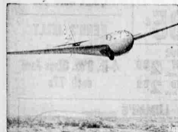
First all-plywood plastic glider, built entirely of wood and other non-strategic materials, lands at Los Angeles after successful test flight. Machine is two-place "transitional" trainer incorporating principal design characteristics of giant cargo gliders soon to come.
