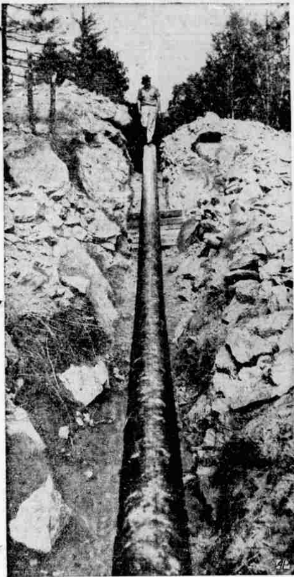
ROCKY ROAD —Solid granite had to give way at Gilead, Me., for this pipe line ditch, part of a 236-mile, $8,000,000, pipe line being built to carry crude oil from Portland, Me., to Montreal, Canada. Oil flow starts about Dec. 1.
