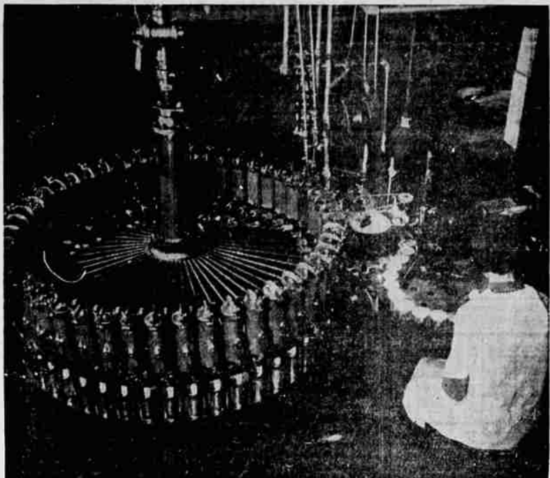
FILLER, where ingenious filling nipple allows milk to flow into can through small hole in bottom of can while air rushes out. A jet of steam spurts across filler hole, solder bar and solder iron drop just one drop of solder over filling hole and cans are conveyed to
