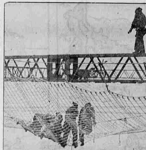
This is a section of the huge life net installed under San Francisco's Golden Gate Bridge to ensure its continuance as "the safest construction job in the world." Workmen are shown installing and testing a section of the net, which will remain in place while the span deck is erected. (Associated Press Photo)
