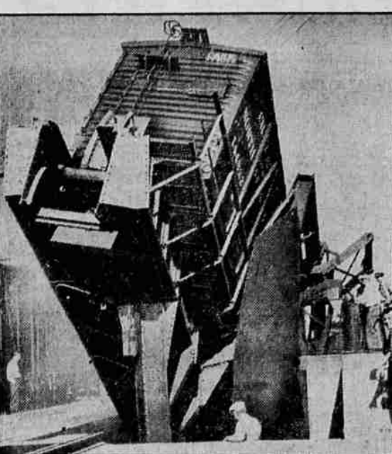
This newly developed car unloader enables a Milwaukee malting company to dump a carload of barley into its elevators in six minutes. The device tips the car up on end and the grain flows into the elevator. Company officials claim it is the only gadget of its kind in the country. (Associated Press Photo)
