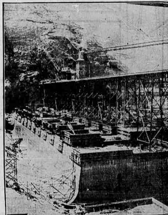
This huge block of concrete will form part of the Grand Coulee dam across the Columbia river in eastern Washington. The octagonal tower in the background is an automatic concrete mixing plant. (Associated Press Photo)
