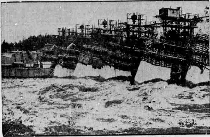
An unusually early spring freshet sent the Columbia river on a rampage which threatened a key crib in the $42,500,000 Bonneville Dam power and navigation project and halted barge operations. Engineers, however, reported no material damage resulted. Here are the raging waters battering against the partially completed dam. (Associated Press Photo)
