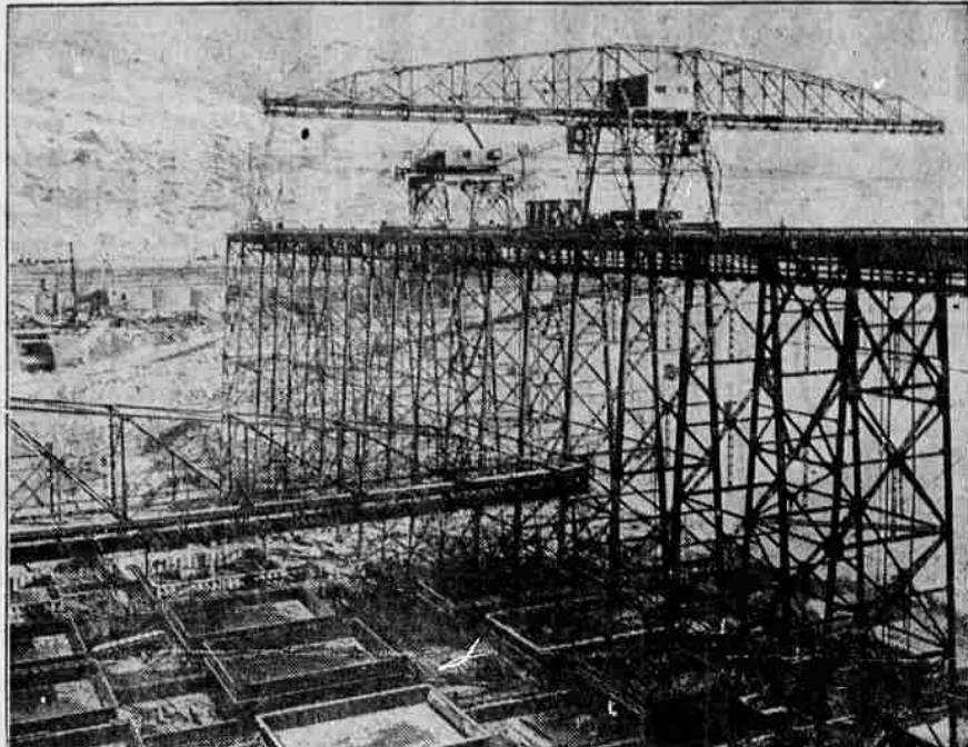
Winter's cold over, pouring of concrete at the Grand Coulee dam project on the Columbia river in Washington has been speeded. The trestle here, nearly 200 feet high, is only a temporary structure for use during the pouring. Mixed concrete is hauled in huge buckets on flat cars from the "House of Magic" mixing plant to the "hammer-head" crane atop the trestle and lowered into the rectangular forms. (Associated Press Photo)
