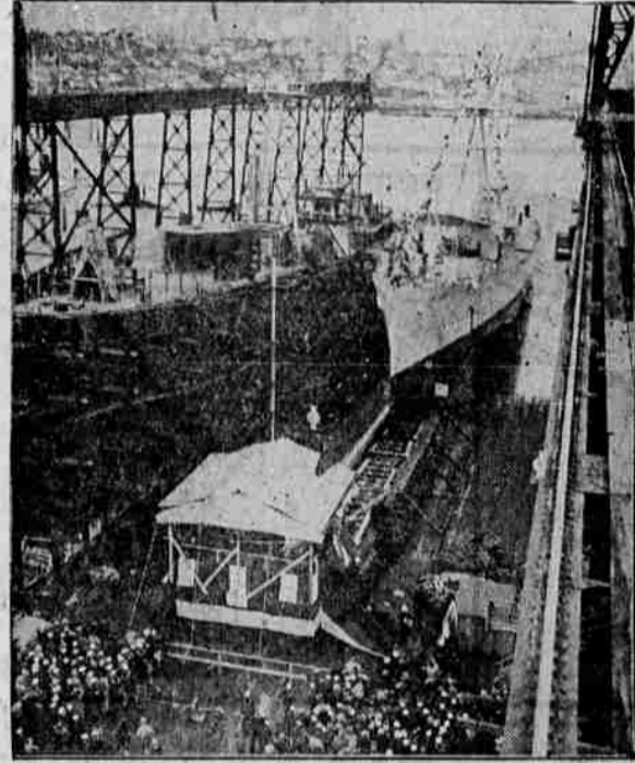
The destroyer Smith, named for a Civil War naval hero, is pictured as it slid down the ways after christening ceremonies before 10,000 persons at the Mare Island Navy Yard. Another destroyer may be seen under construction alongside. (Associated Press Photo)
