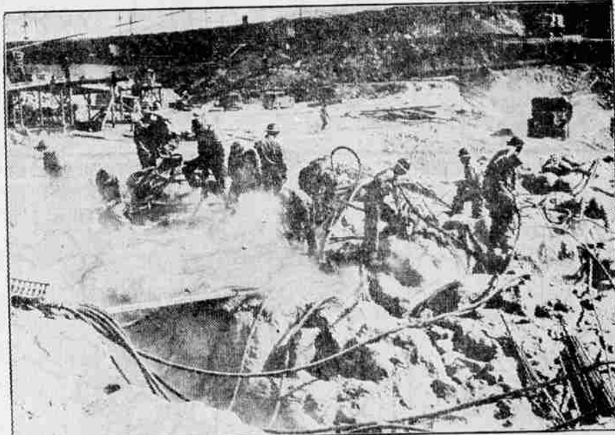
A jackhammer crew at work on the bedrock of the west excavation of the Grand Coulee dam on the Columbia river in Washington. They are drilling preparatory to placing a blast that will prepare the rock for the dam's foundation. (Associated Press Photo)
