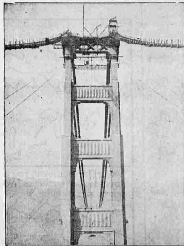
Preparations for spinning the cables of the Golden Gate bridge between Marin county and San Francisco occupied crews today. They were busy erecting storm cable system, telephone system and various units of the spinning equipment for the $35,000,000 structure. The cable, stretching from the tower in the foreground to the Marin county on north side, will be 36 1/2 inches in diameter. The catwalks with some of the storm cables is shown. (Associated Press Photo)
