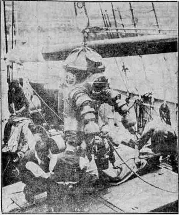
An all-metal diving suit being lowered into the hold of the salvage ship "Ophir" in the River Clyde in Glasgow, Scotland, which was to be used in an effort to reach the Lusitania, sunk by U-boats off the coast of Ireland on the eve of America's entry into the World War. (Associated Press Photo)
