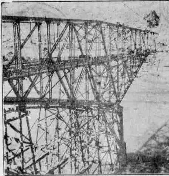
Here's a view of the new highway bridge being built across the Columbia river at the Grand Coulee dam site in Washington. The bridge is being built as part of the bureau of reclamation's construction program there. (Associated Press Photo)
