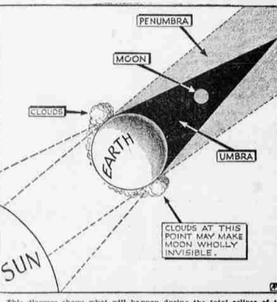
This diagram shows what will happen during the total eclipse of the moon on the night of July 15-16. Because of light rays bent by the atmosphere at the earth's edge, the moon will be slightly visible even in total shadow unless clouds interfere with its refracted light.
