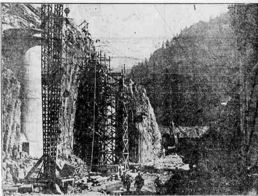
This view shows how construction is progressing on the $3,000,000 navigation locks at the $34,000,000 Bonneville dam on the Columbia river near Portland, Ore. Sea-going freighters will pass through here to the wharves that will line the wide lake formed by the dam. (Associated Press Photo)
