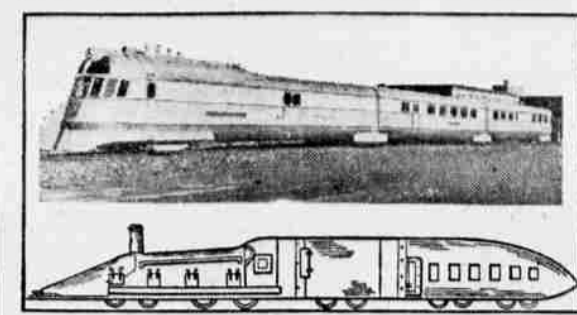
(Above) One of the new stainless steel, streamlined Zephyrs just completed for the Burlington Railroad. (Below) Drawing of the streamlined train for which a patent was granted by the U. S. Patent Office to Samuel R. Calthrop, of Roxbury, Mass., in 1865.
