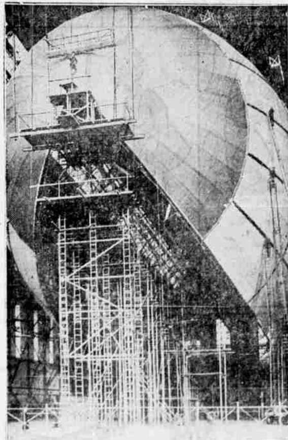
Germany's latest bid for supremacy in the air, the new zeppelin LZ-129, which is scheduled to inaugurate passenger and mail service between Germany and the United States, is shown in its hangar at Friedrichshafen where it is rapidly nearing completion. (Associated Press Photo)
