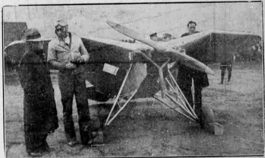
This tiny airplane, one of the smallest ever built, attracted attention at the dedication of the Troy, N. Y., airport. The "motorized mosquito" was built by Edward H. Lanier (left) and flown by Wendell Fleming (right). It has a wing spread of 14 feet and is 16 feet long. The builder claims it will fly 250 miles on eight gallons of gasoline. (Associated Press Photo)
