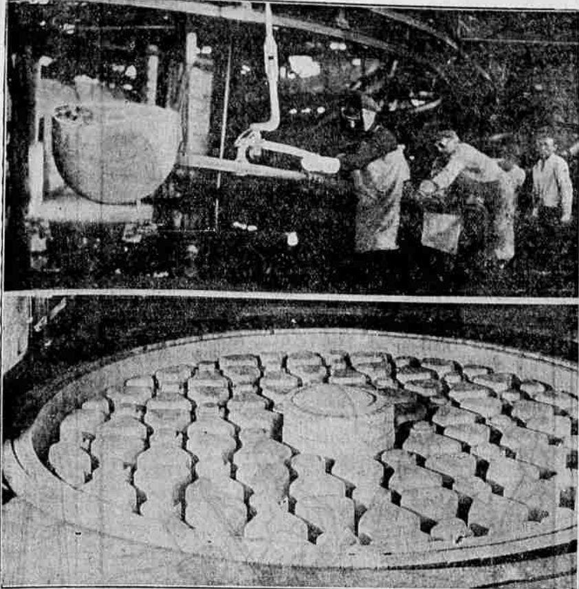
The pouring of 20 tons of molten glass to form the "eye" of the world's largest telescope took place at Corning, N. Y. In what was regarded as an epochal step in scientific achievement, the mold of the "eye," or mirror, of the 200-inch telescope is shown below. Above is a huge iron ladle from which the glass was poured. The crew leader is helmeted against glare. It took a month to heat the glass and it will take 10 months to cool it. (Associated Press Photos)
