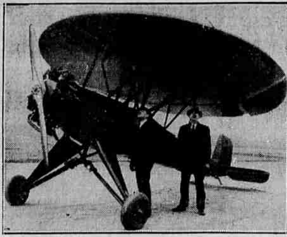
This odd plane with a round disc for wings was hailed by inventors as a step forward in the hunt for a plane that will land in limited space. It is designed to go 135 miles an hour and to land at a 60-degree angle in a 25-foot circle. Picture was made when the ship was being tested in Chicago. (Associated Press Photo)
