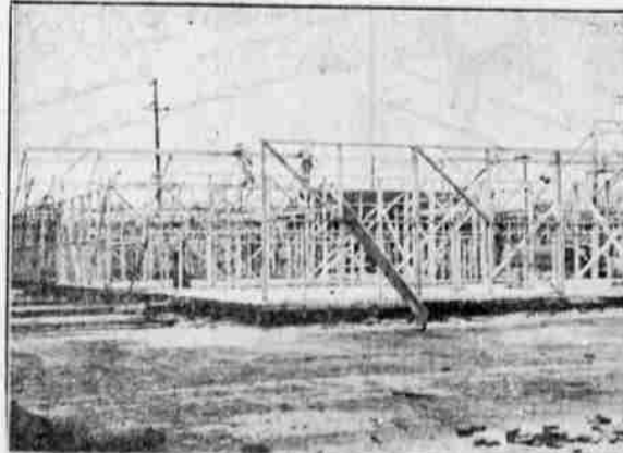
Workmen erecting tent schools in Berkeley, Cal., to take the place of three schools there which have been condemned as earthquake hazards. The tents will be steam-heated. There will be wood frames, floors and sidewalls four feet high, the remainder being canvas. (Associated Press Photo)
