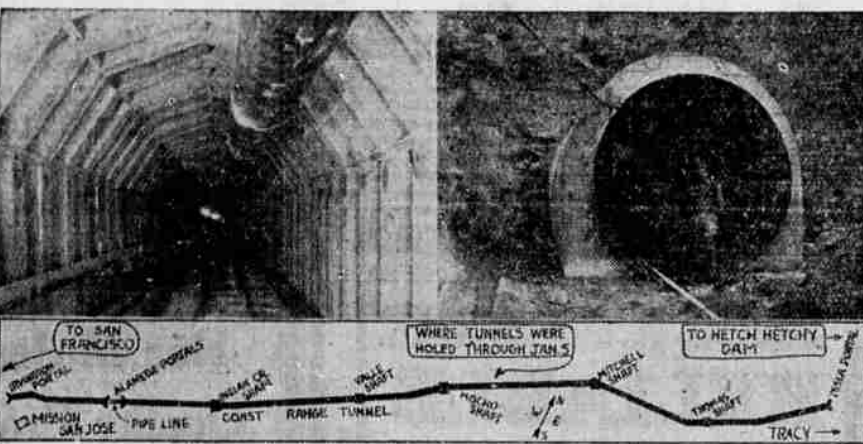
Two views of the coast range tunnel which was "holed through" Jan. 5. The tunnel, said to be the longest in the world, is 28.6 miles in length, 25.1 of them being continuous from the Tesla portal to the East Alameda portal. At left is a section of the tunnel as it appears completed and (right) the Irvington portal near Mission San Jose. The map shows the route of the huge tunnel which will convey water from Hetch Hetchy dam high in the Sierra Nevada mountains to San Francisco. In all there are 167 miles of aqueduct. (Associated Press Photo)
