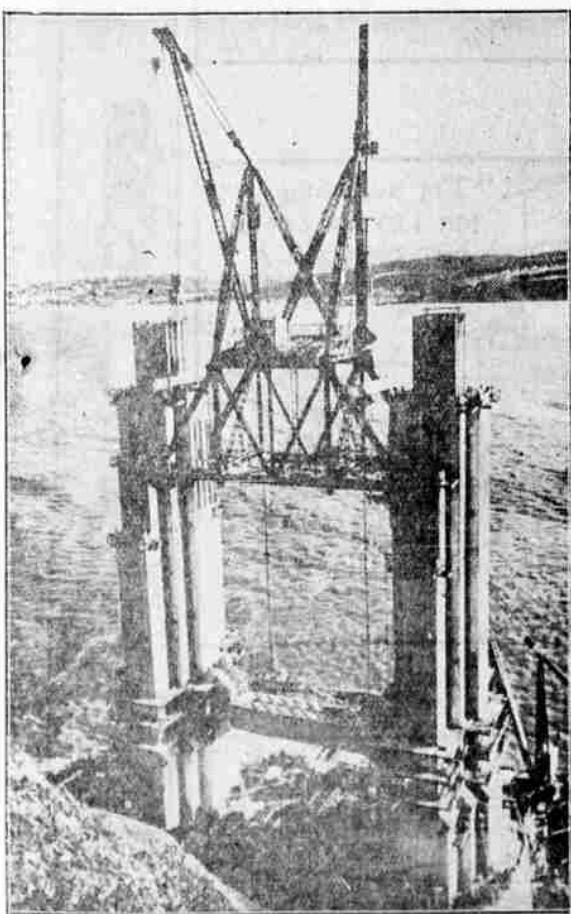
The Marin county tower of the Golden Gate bridge connecting San Francisco with the north is shown as it nears completion. The tower has reached a height which approximates the floor of the bridge. A creeper truss is shown at the top while the huge cross truck below will serve as a permanent tie between the two tower legs. (Associated Press Photo)
