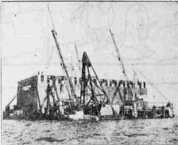
Measuring 92 feet wide and 197 feet long, a caisson was towed into San Francisco bay and floated into position as the first step in building the center anchorage of the San Francisco-Oakland bridge. The caisson, the largest in the world, will be used to build a great pier that will stand 298 feet above the waterline. (Associated Press Photo)
