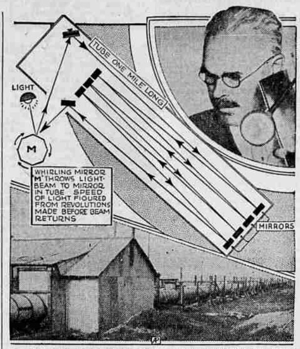
Dr. Francis G. Pease (above) of the Carnegie Institution's Mt. Wilson observatory, and Dr. Fred Pearson of the University of Chicago are using a mile-long tube (below) incorporating an arrangement of mirrors reflecting light from a whirling mirror (diagram) to make further checks on the speed of light.
