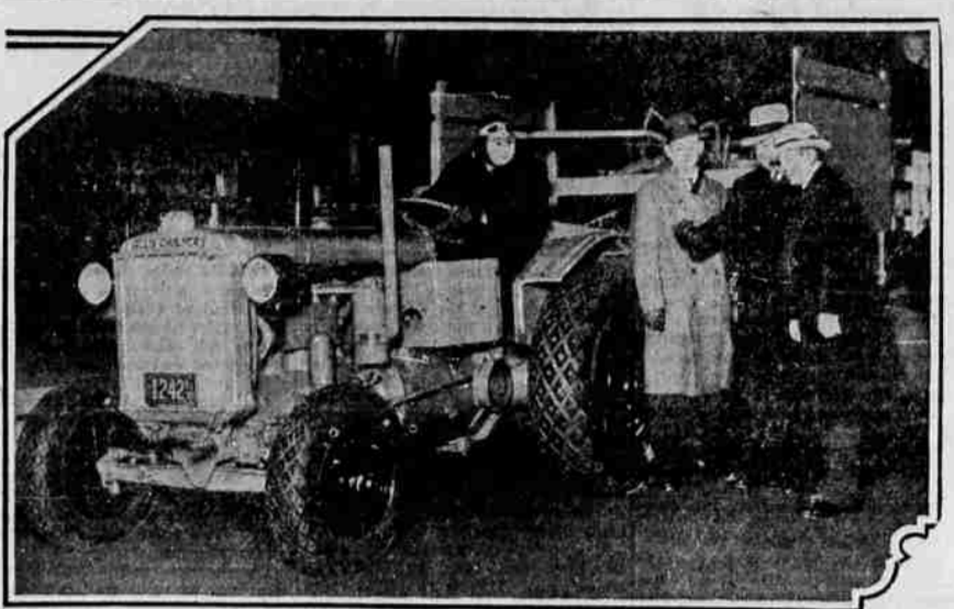
Goodyear pneumatic Farm Tractor tires applied to this Allis Chalmers tractor made possible its speedy trip, the first ever attempted by a tractor and trailer, from Milwaukee to Chicago with a load of implements for the International Livestock show. The tractor traveled through city streets and even down Chicago's Michigan avenue, where a steel wheeled tractor would have been ruled off.
