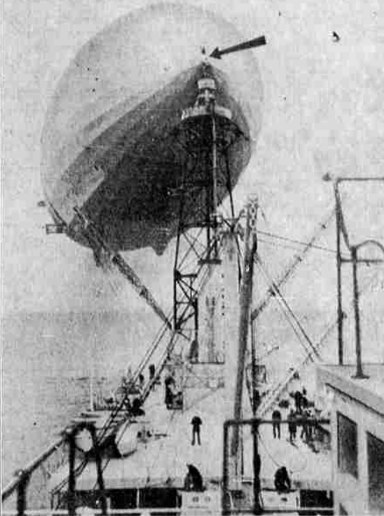
The U.S.S. Akron photographed the instant she was moored to the U.S.S. Patoka, her mothership, in San Francisco bay. Arrow indicates one of the most hazardous jobs, that of a sailor on top of the mooring mast who fits the tangle of the Akron's nose into a socket. Immediately above him is a flying sailor who lets down the mooring lines.
